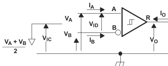
Figure 7-9. Receiver DC Parameter Definitions
