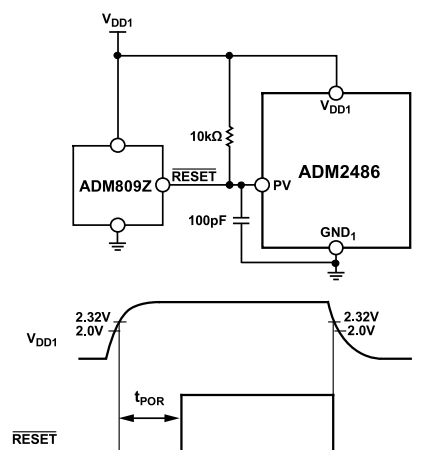
Figure 31. Driving PV with an Open-Drain Output
