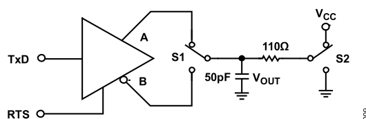
Figure 9. Driver Enable/Disable
