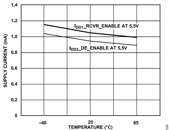
Figure 16. Unloaded Supply Current vs. Temperature
