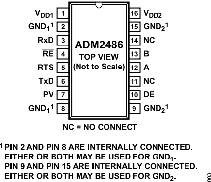
Figure 2. Pin Configuration
