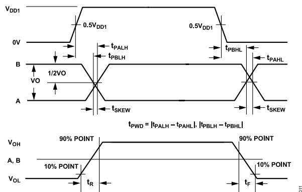
Figure 12. Driver Propagation Delay, Rise/Fall Timing
