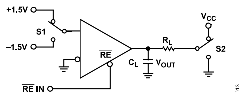
Figure 11. Receiver Enable/Disable
