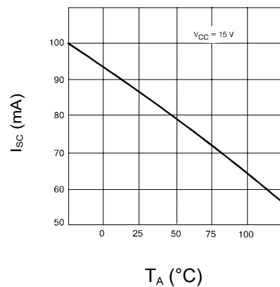
Figure 6: Reference Short Circuit Current vs. Temperature
