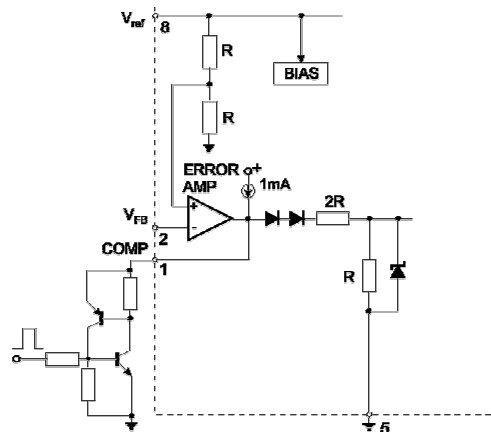
Figure 5. Latched Shutdown
