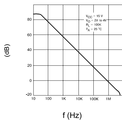
Figure 4: Error Amp Open-Loop Gain vs. Frequency
