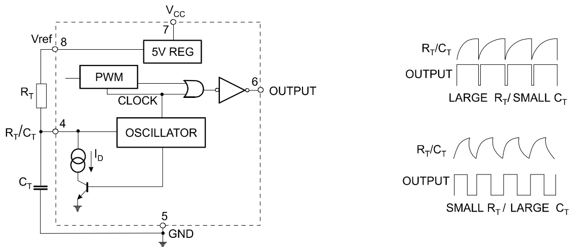
Figure 9. Oscillator and Output Waveforms
