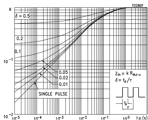
Figure 14. Normalized transient thermal impedance
