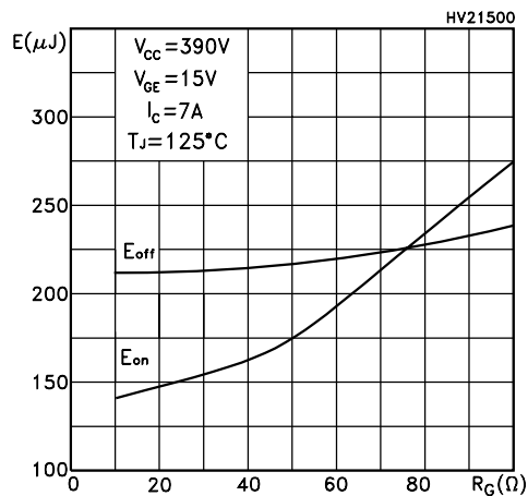
Figure 12. Typical switching energy vs gate resistance
