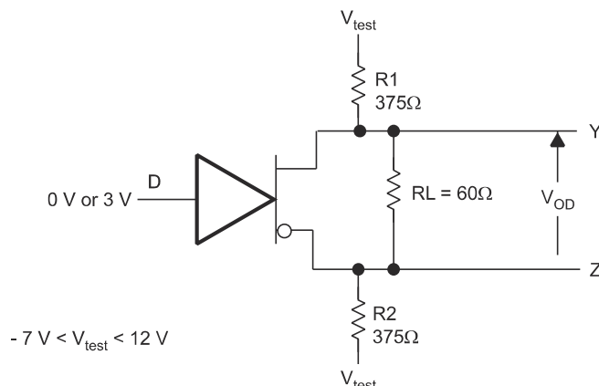
Figure 6-2. Driver V_{OD3}
