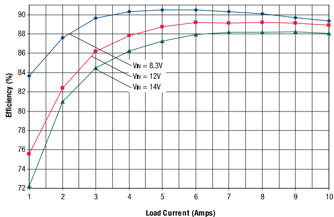
OKY2-T/10-D12 Efficiency vs. Line Voltage and Load Current @ +25°C (V OUT = 1.8V)
