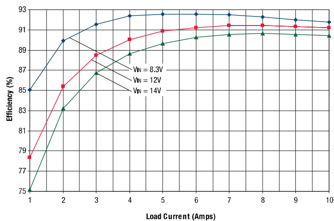
OKY2-T/10-D12 Efficiency vs. Line Voltage and Load Current @ +25°C (V OUT = 2.5V)
