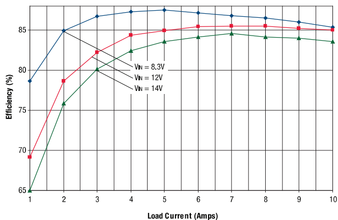
OKY2-T/10-D12 Efficiency vs. Line Voltage and Load Current @ +25°C (V OUT = 1.2V)
