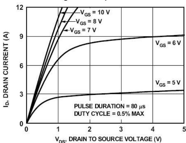
Figure3. Output characteristics
