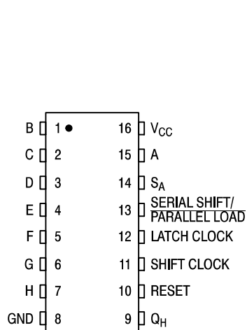
Figure 1. Pin Assignment
