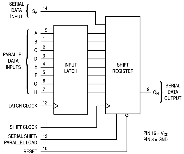
Figure 2. Logic Diagram
