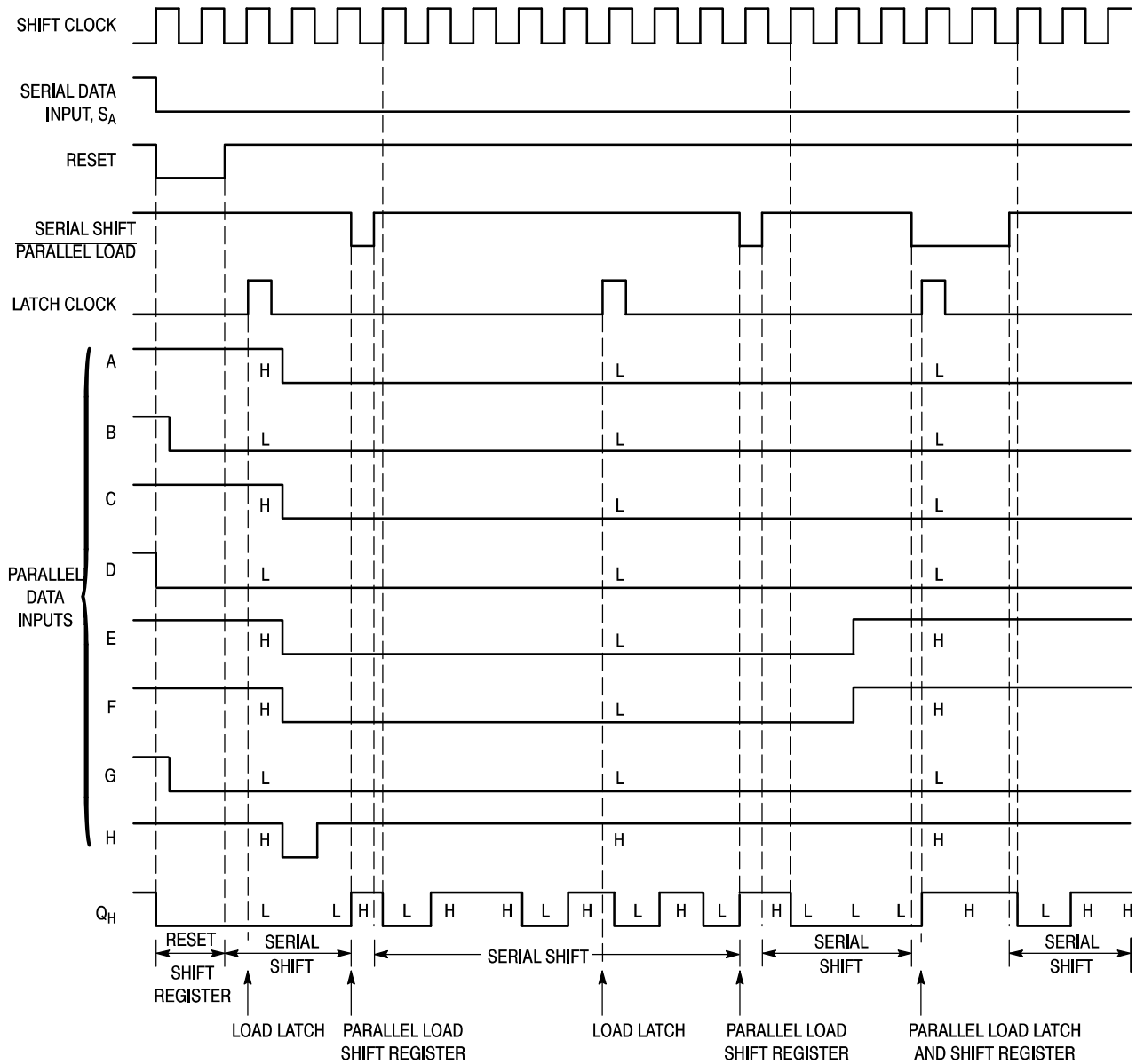
Figure 12. Timing Diagram
