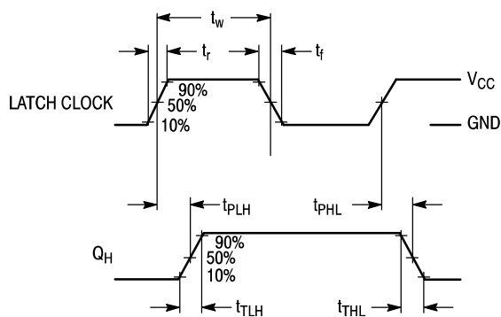
Figure 4. (Serial Shift/Parallel Load = L)
