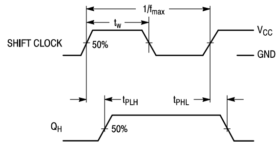
Figure 5. (Serial Shift/Parallel Load = H)
