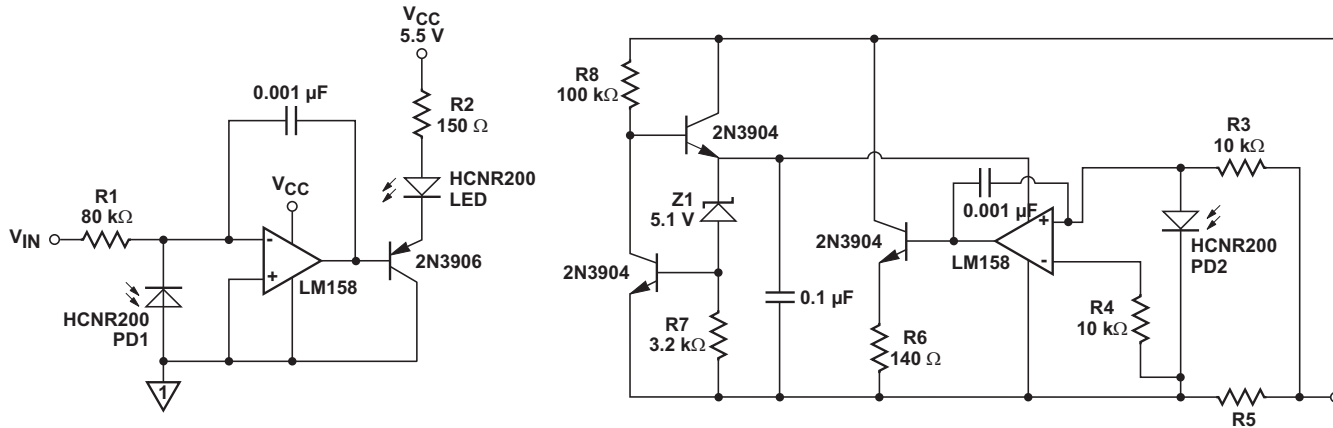
Figure 23: 4 mA to 20 mA HCNR200 Transmitter Circuit
