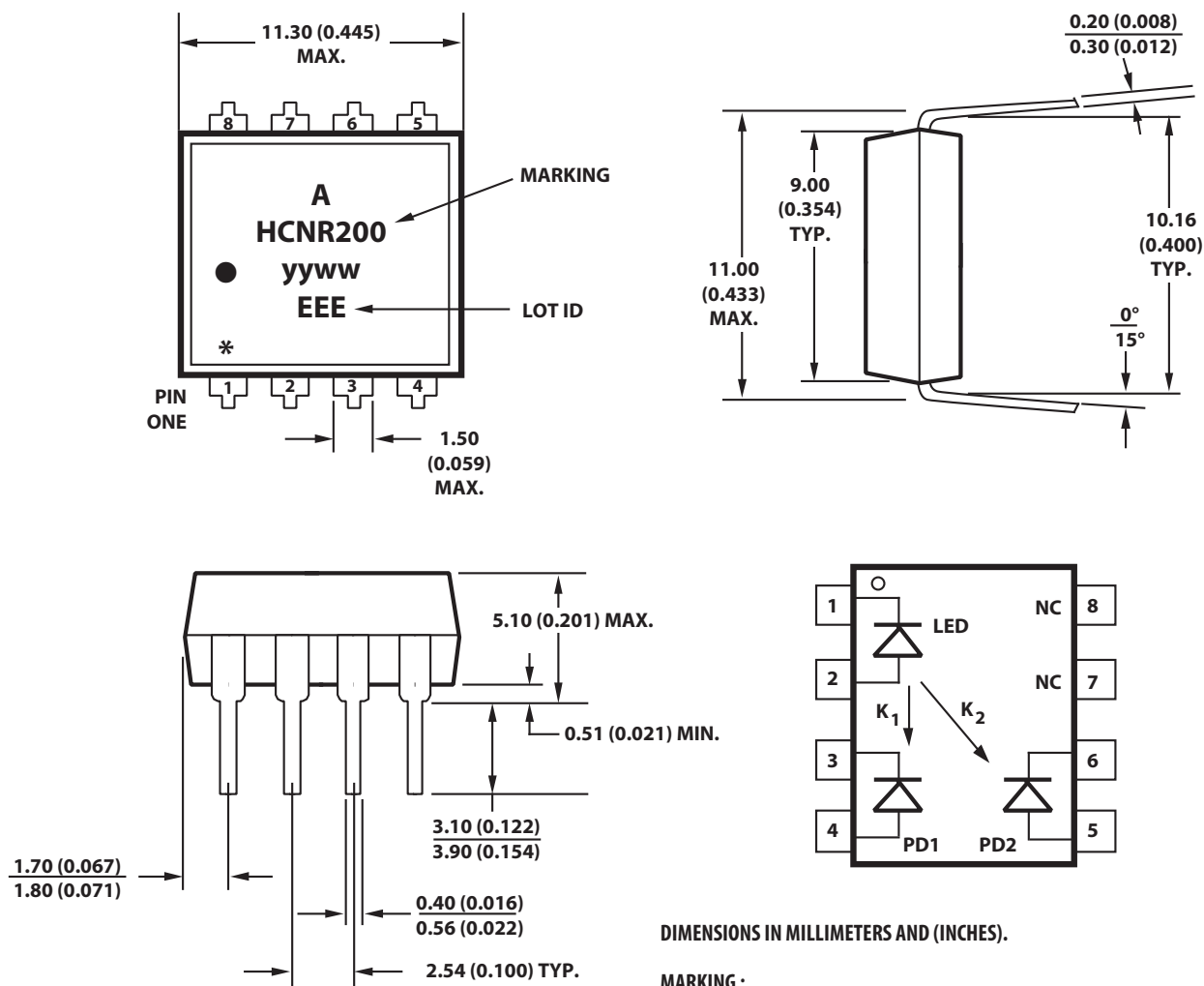
Figure 1: 8-Pin DIP
