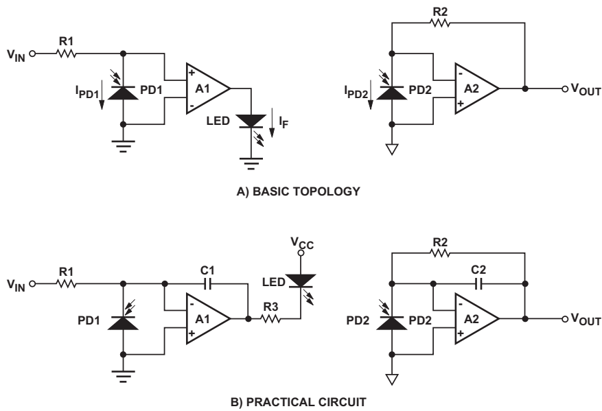
Figure 14: Unipolar Circuit Topologies
