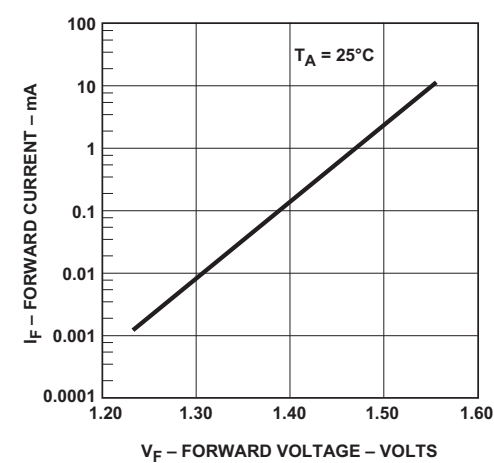
Figure 10: LED Input Current vs. Forward Voltage
