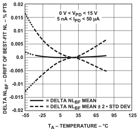
Figure 7: NL_{BF} Drift vs. Temperature
