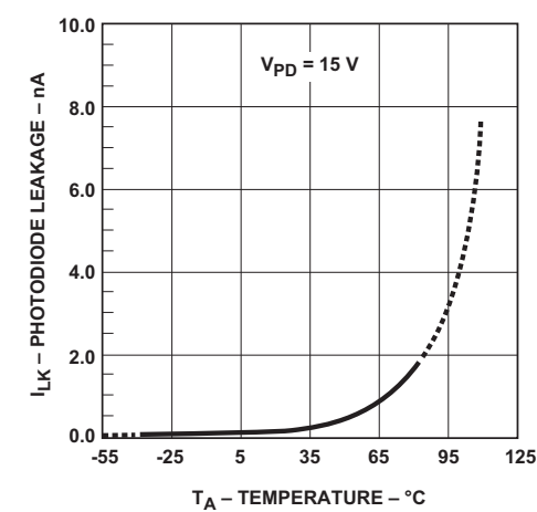
Figure 9: Typical Photodiode Leakage vs. Temperature
