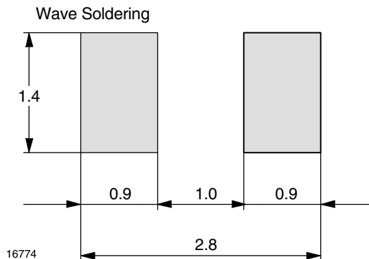
Fig. 10 - Recommended Foot Pads (in mm)
