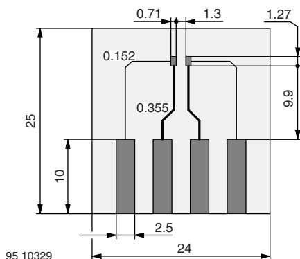
Fig. 8 - Board for R_{thJA} Definition (in mm)
