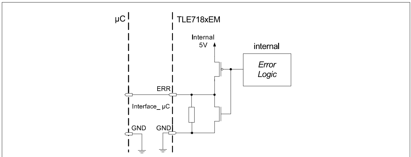
Figure 4 Structure of \overline{\text{ERR}} output
