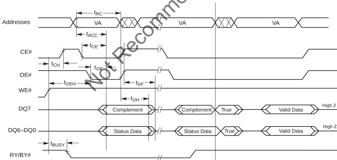
Figure 15.7 Data# Polling Timings (During Embedded Algorithms)
