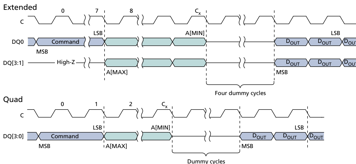
Figure 23: QUAD INPUT/OUTPUT WORD READ – E7h 3
