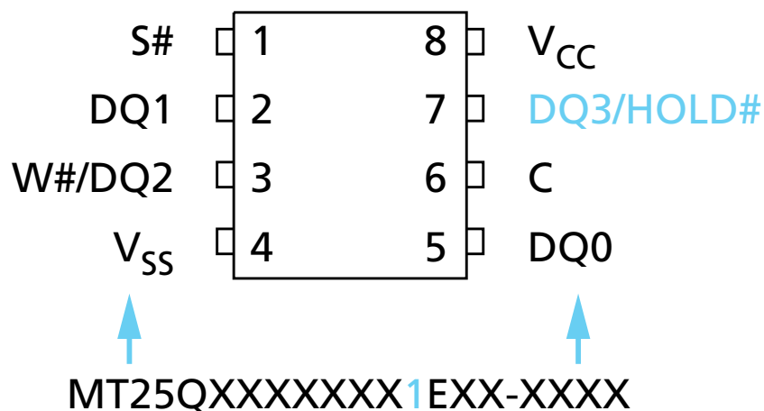
Figure 6: 8-Pin, SOP2 or W-PDFN (Top View)
