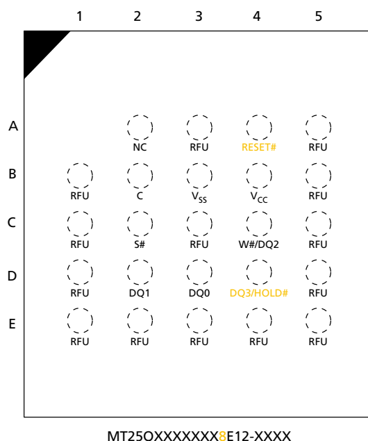
Figure 4: 24-Ball T-BGA, 5 x 5 (Balls Down)
