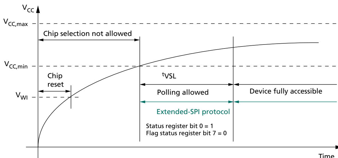
Figure 46: Power-Up Timing
