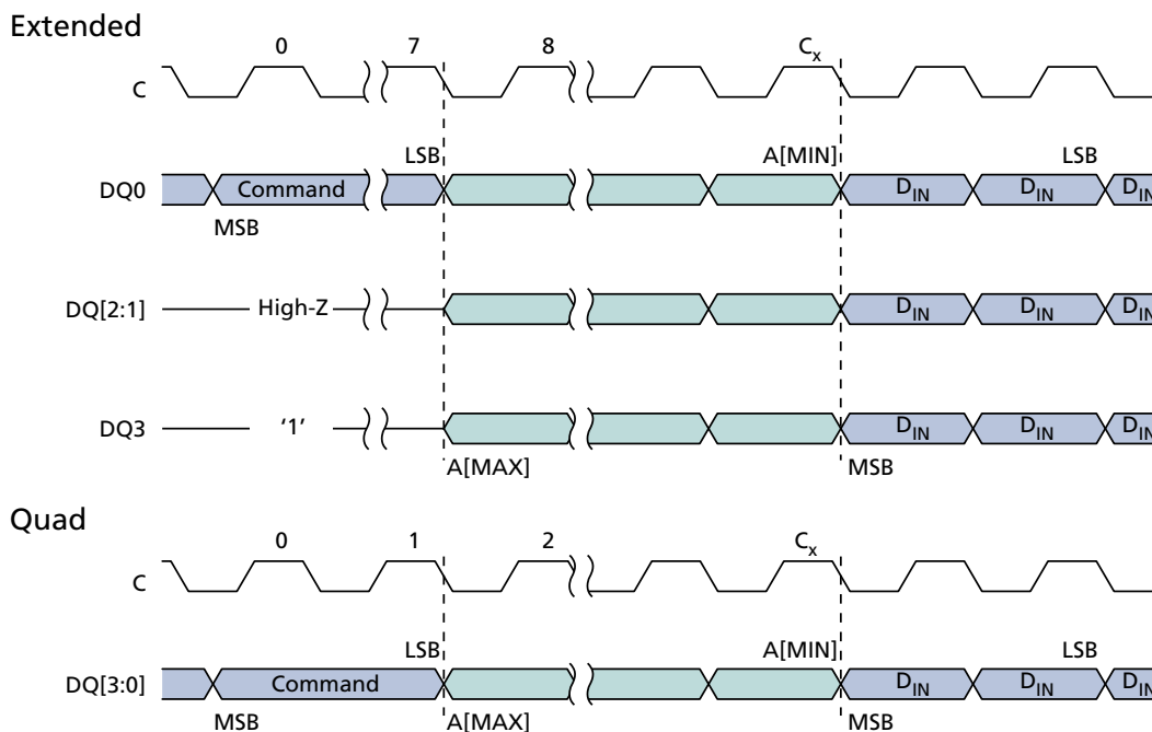
Figure 37: EXTENDED QUAD INPUT FAST PROGRAM Command
