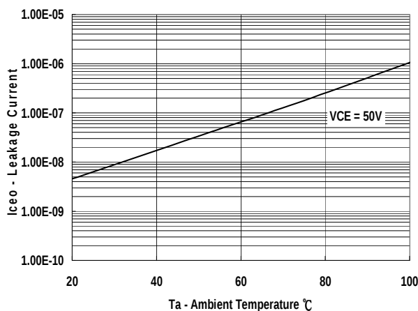
Figure6. Collector Leakage Current vs. Ambient Temperature
