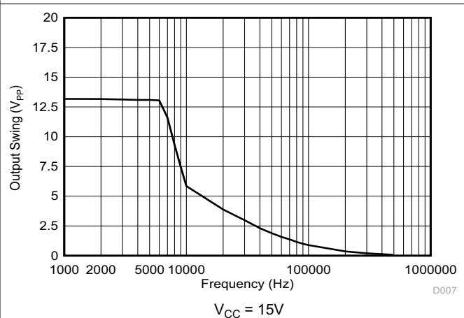
Figure 6-40. Maximum Output Swing vs Frequency
