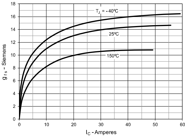
Fig. 7. Transconductance
