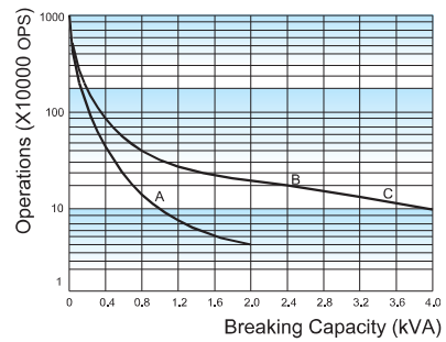
ENDURANCE CURVE(Resistive)
