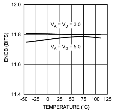
Figure 29. ENOB vs Temperature
