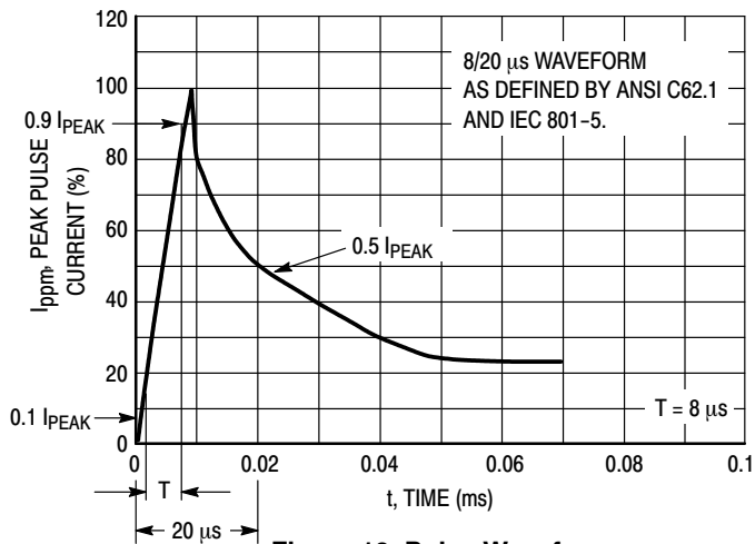
Figure 10. Pulse Waveform
