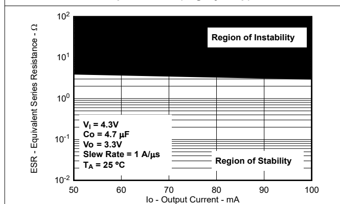
Figure 5-48. TPS76933 Typical Regions of Stability ESR vs Output Current (Legacy Chip)
