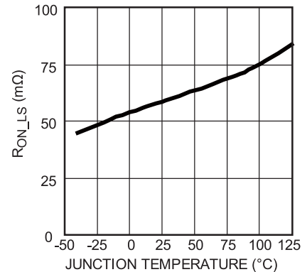
R_{ON-LS} vs. Junction Temperature
