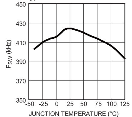
F_{sw} vs. Junction Temperature
