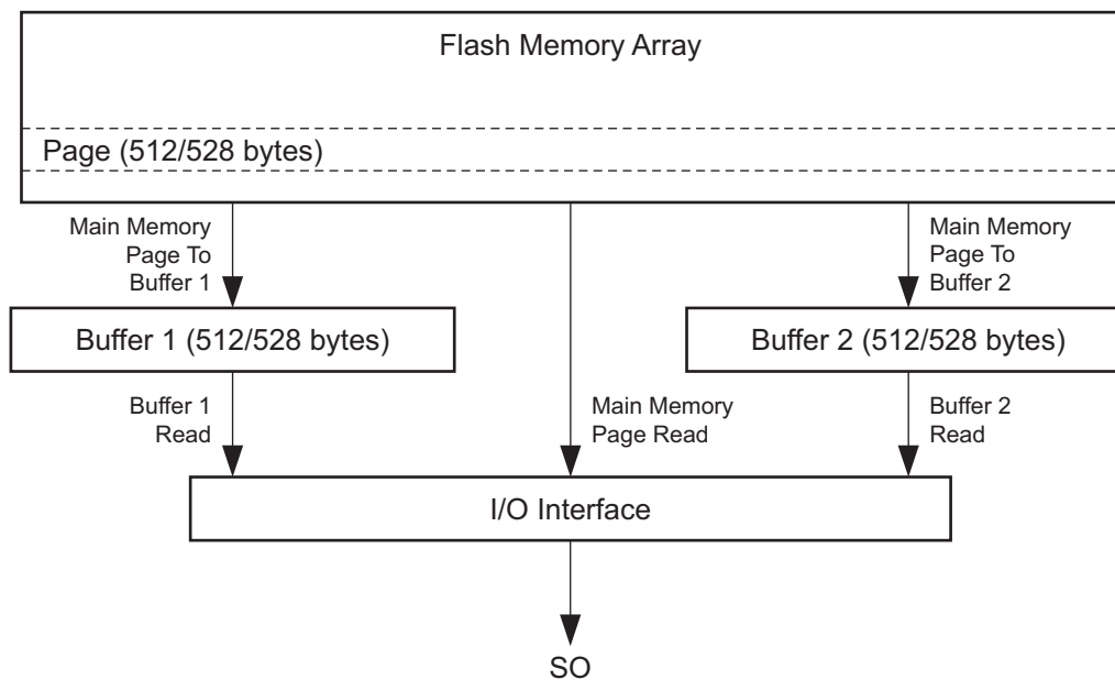
Figure 34. Block Diagram
