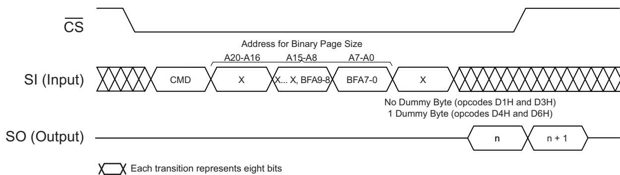
Figure 37. Buffer Read
