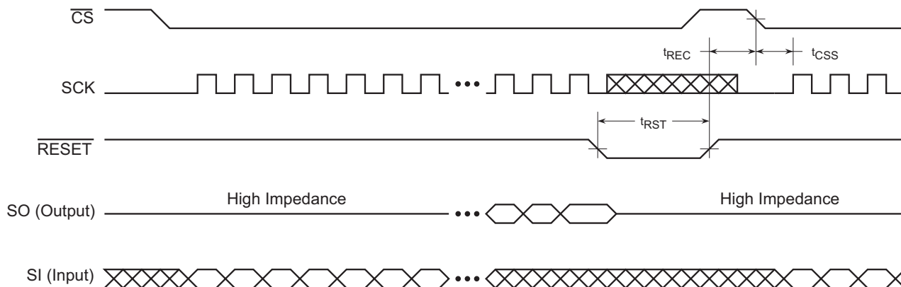
Figure 49. Reset Timing
