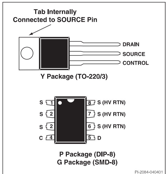
Figure 3. Pin Configuration.
