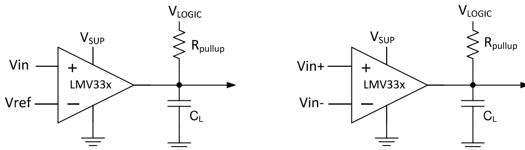
Figure 7-1. Typical Application Schematic
