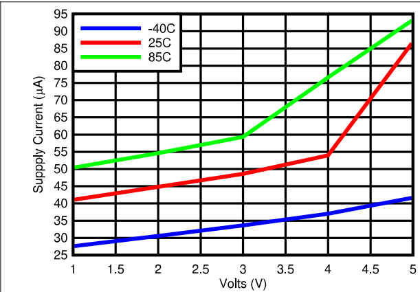
Figure 5-2. Supply Current vs Supply Voltage Output Low
