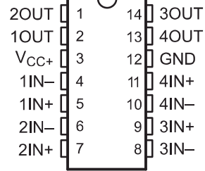
LMV339 . . . D OR PW PACKAGE (TOP VIEW)
