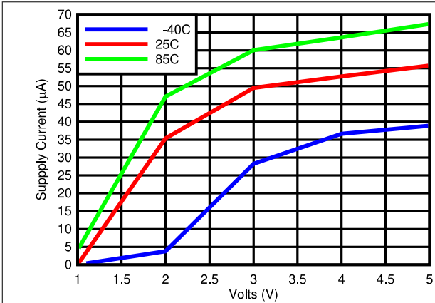
Figure 5-1. Supply Current vs Supply Voltage Output High
