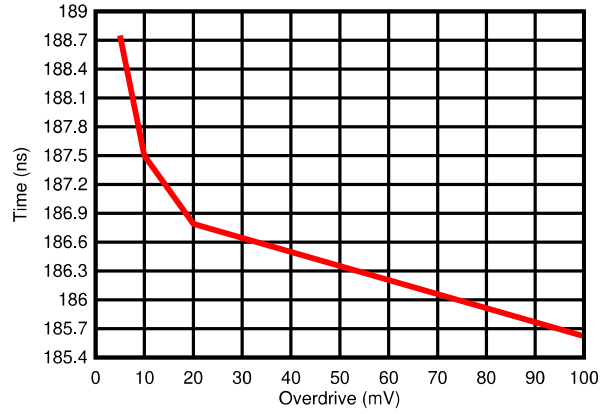
Figure 5-8. Response Time vs Input Overdrives Positive Transition ( V_{CC} = 2.7V )
