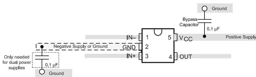
Figure 9-1. LMV331 Layout Example
