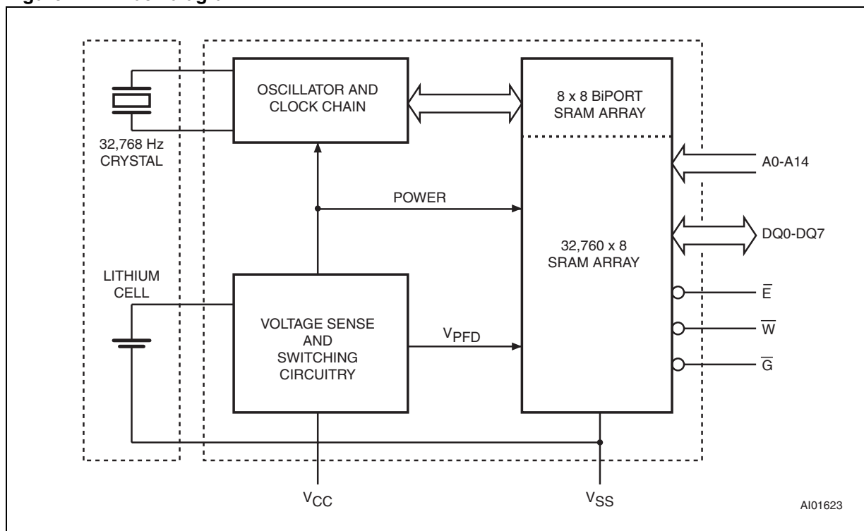
Figure 4. Block diagram
