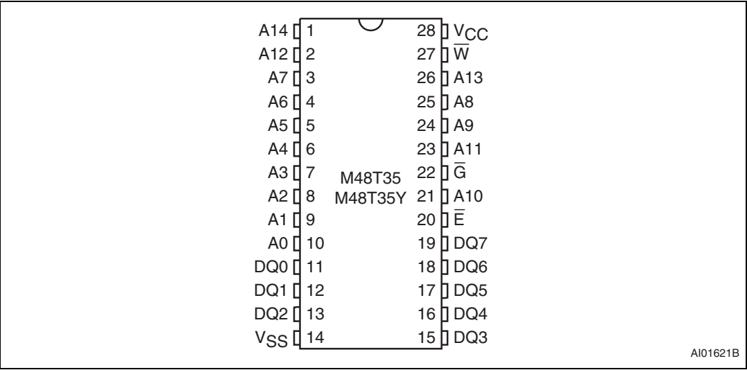
Figure 2. DIP connections
