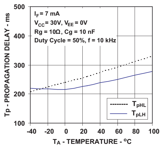
Figure 13: Propagation Delay vs. Temperature
