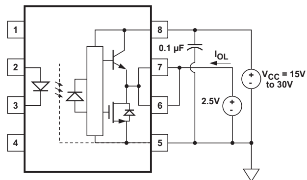
Figure 17: I_{OL} Test Circuit
