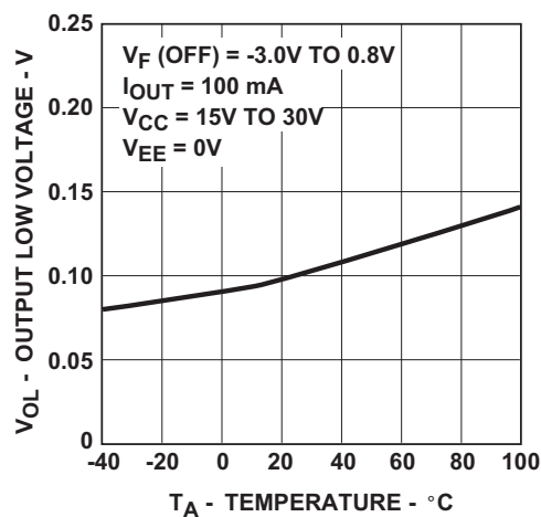
Figure 5: V_{OL} vs. Temperature
