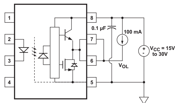
Figure 19: V_{OL} Test Circuit
