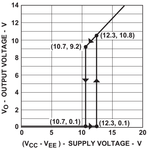
Figure 15: Undervoltage Lockout
