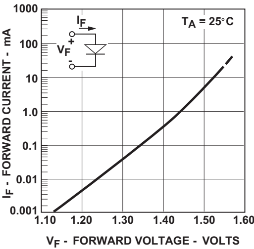
Figure 14: Input Current vs. Forward Voltage
