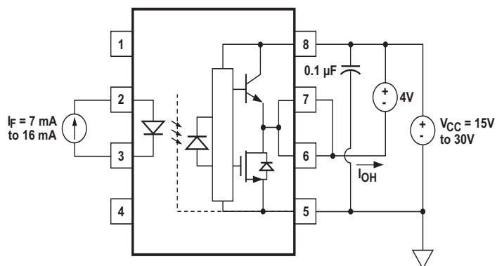
Figure 16: I_{OH} Test Circuit
