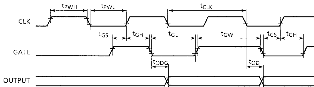
Figure 12.3 Clock &amp; Gate Timing
