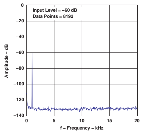
Figure 14. Output Spectrum
