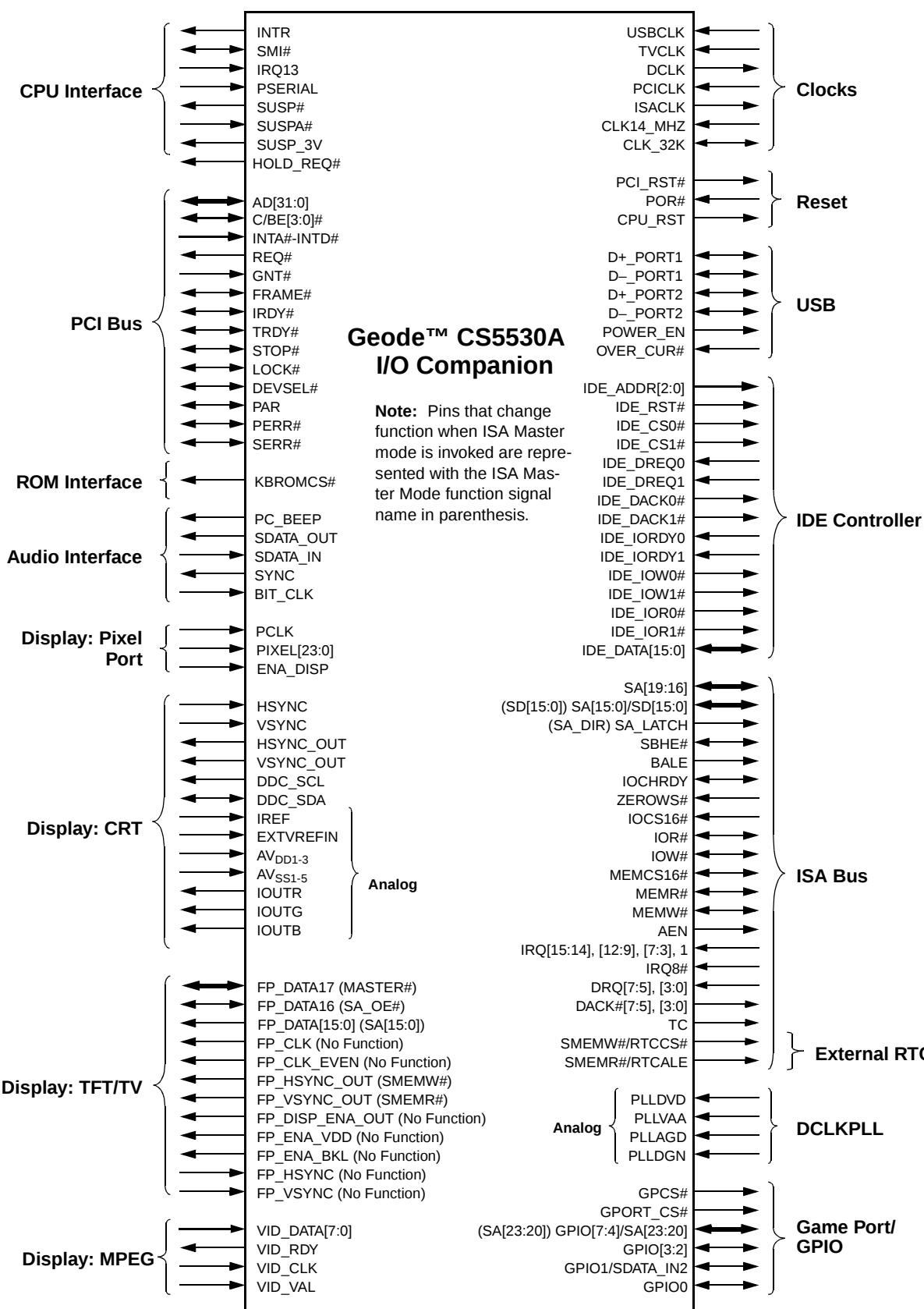
Figure 2-1. CS5530A Signal Groups
