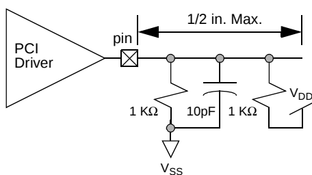
Figure 5-5. PCI Slew Rate Test Circuit
