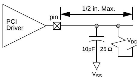
Figure 5-4. PCI Falling Edge ( t_{HL} ) Test Circuit
