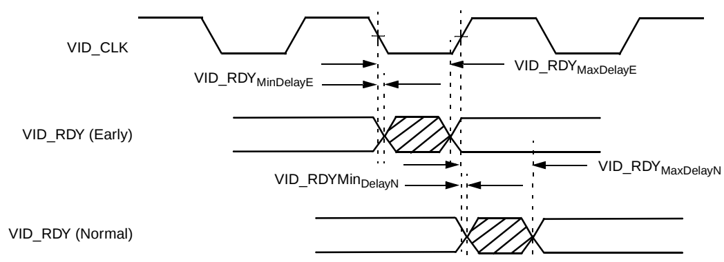
Figure 5-12. MPEG Timing
