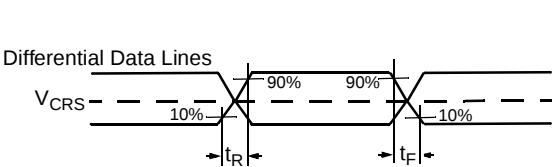
Figure 5-9. USB Timing
