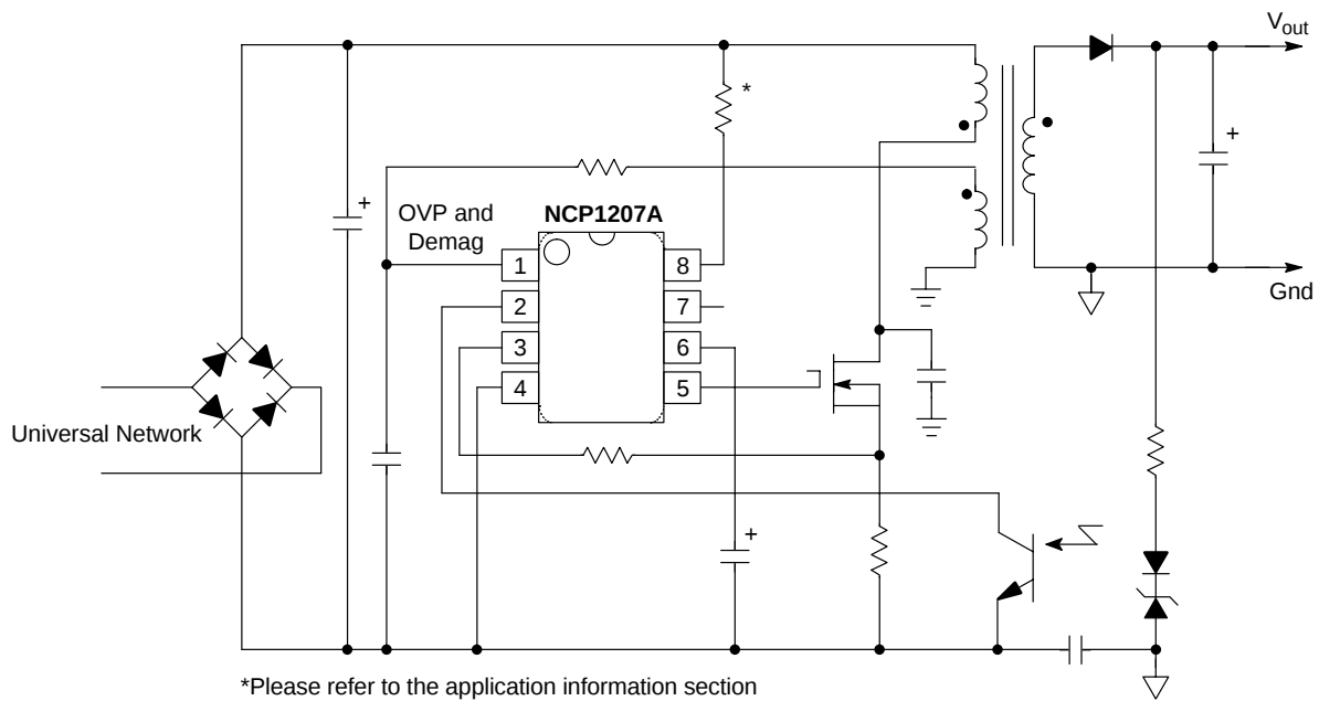
Figure 1. Typical Application
