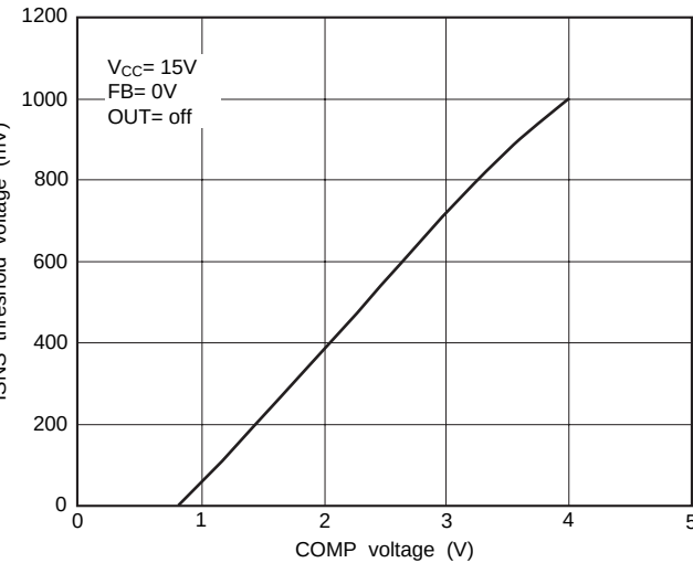
ISNS threshold voltage vs. COMP voltage
