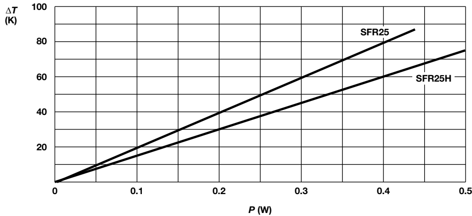
SFR25/SFR25H Hot-spot temperature rise ( \Delta T ) as a function of dissipated power
