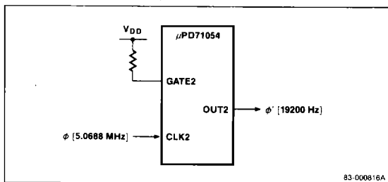
Figure 15. Frequency Division
