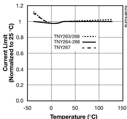
Figure 24. Current Limit vs. Temperature.
