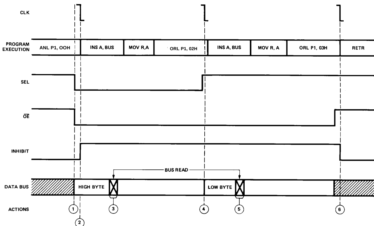
Figure 19. 8748 READ Cycle from Figure 18.
