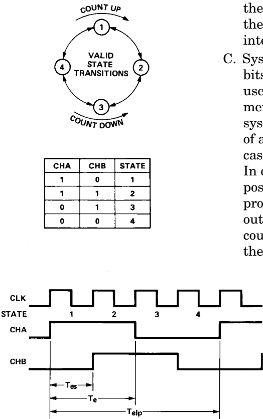
Figure 9. 4x Quadrature Decoding.
