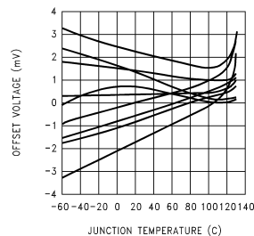
V_{OS} vs Junction Temperature
