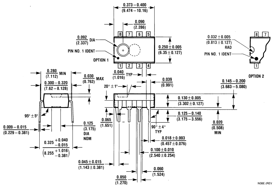
Plastic Dual-In-Line Package (N) Order Number LM611CN, LM611AIN, LM611BIN, LM611AMN or LM611MNN NS Package Number N08E
