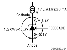
FIGURE 1. Voltages Associated with Reference (Current I_r is External)
