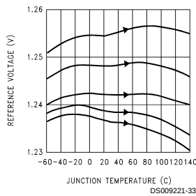
Reference Voltage vs Temp on 5 Representative Units
