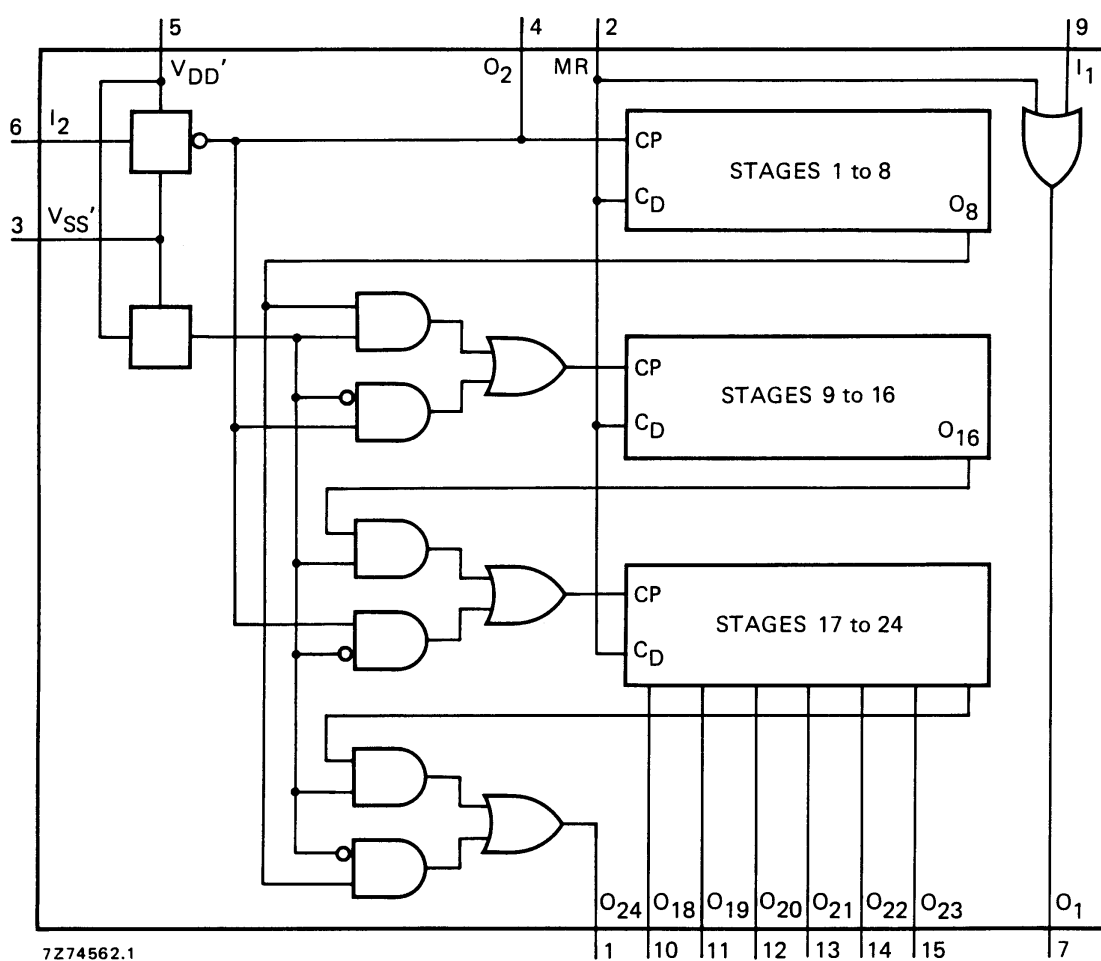
Fig.1 Functional diagram.
