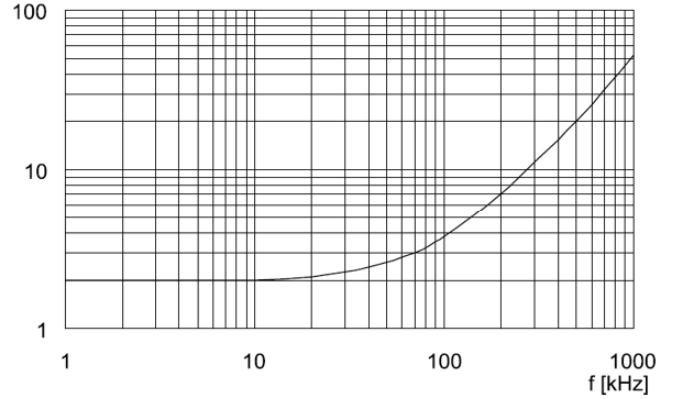
损耗频率特性曲线(室温) Dissipation factor vs. frequency (Room temperature)
