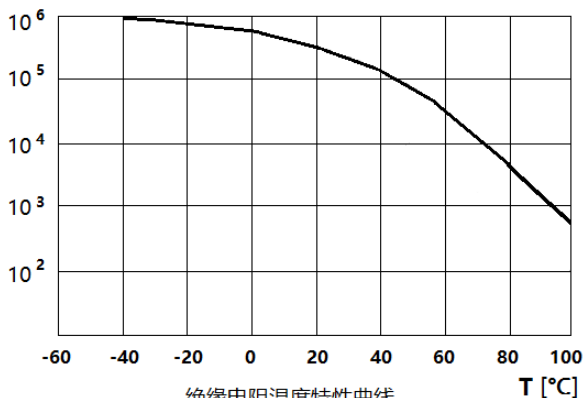
绝缘电阻温度特性曲线 Insulation resistance vs. temperature
