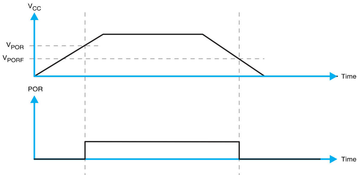
Figure 23. V_{POR}
