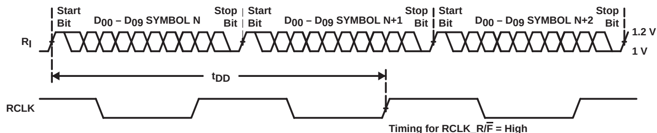
Figure 11. Serializer Delay
