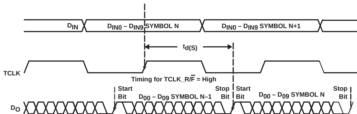
Figure 11. Serializer Delay
