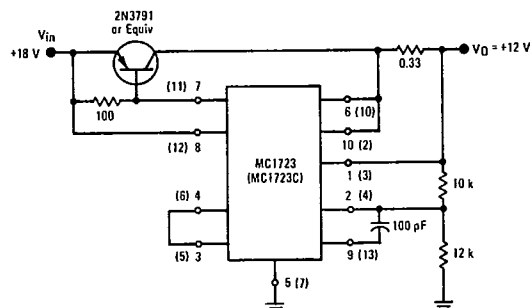
FIGURE 22 - +12 V, 1-AMPERE REGULATOR
