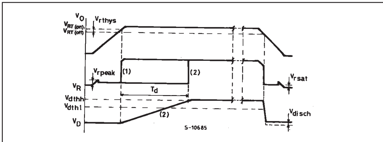
Figure 2: Reset Waveforms:
