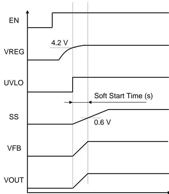
Figure : Soft Start Operation
