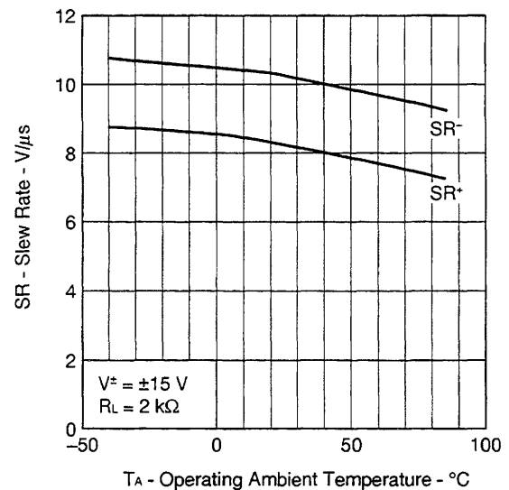
★ SLEW RATE
