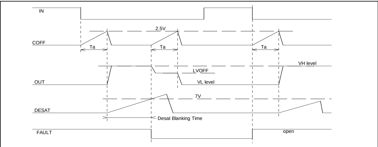
Figure 5: Desaturation fault
