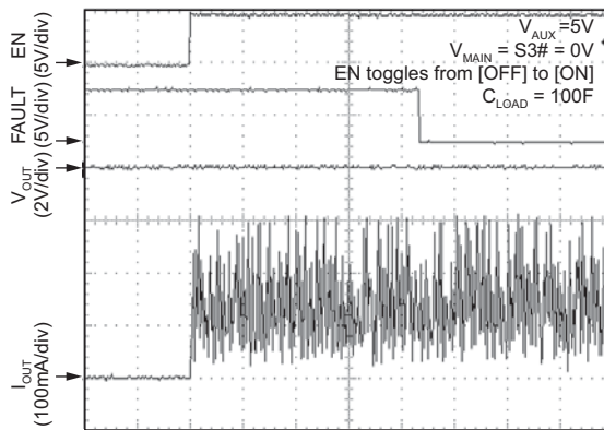
AUX Turn-On into Short
