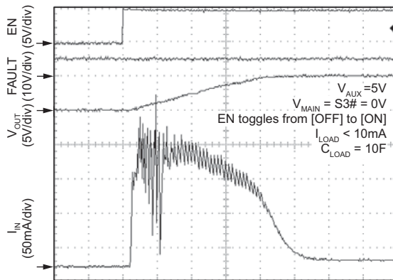
AUX Inrush Current into Small C_{LOAD}
