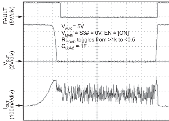
AUX Ramped to Short by MOSFET
