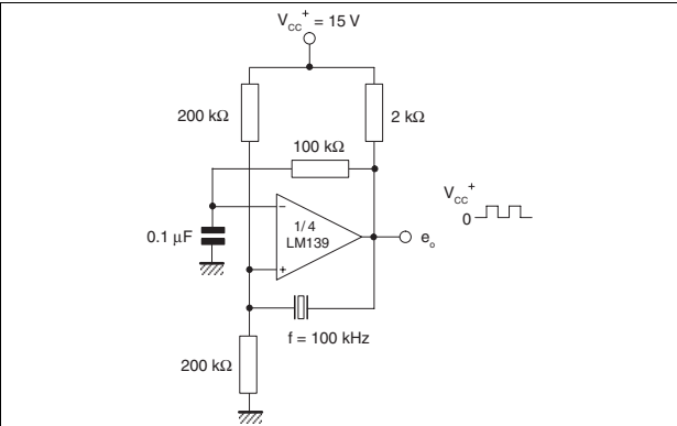
Figure 19. Crystal-controlled oscillator
