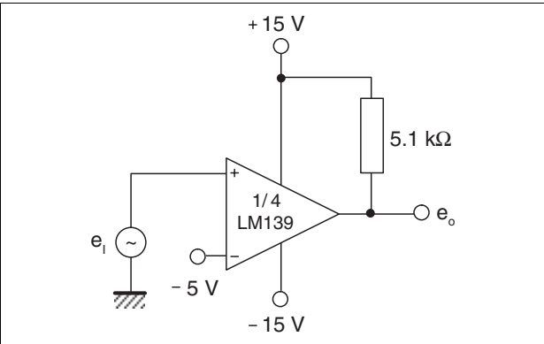
Figure 21. Comparator with a negative reference
