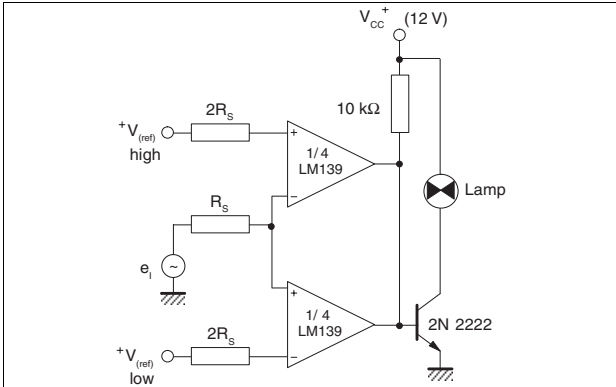
Figure 18. Limit comparator
