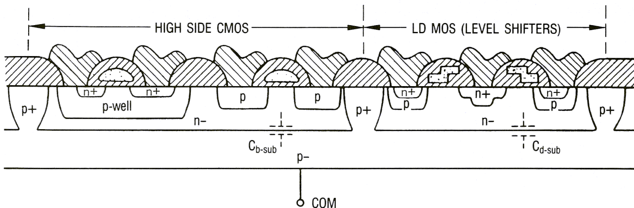
Figure 3. Silicon crossection showing the parasitic capacitances
