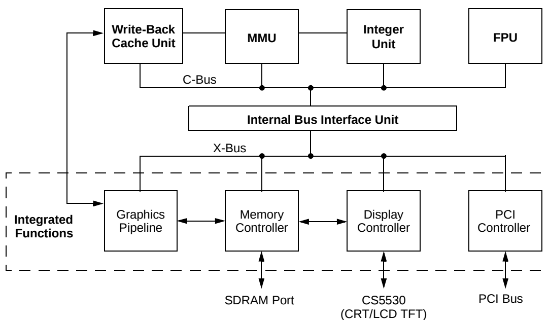
Figure 1-1. Internal Block Diagram
