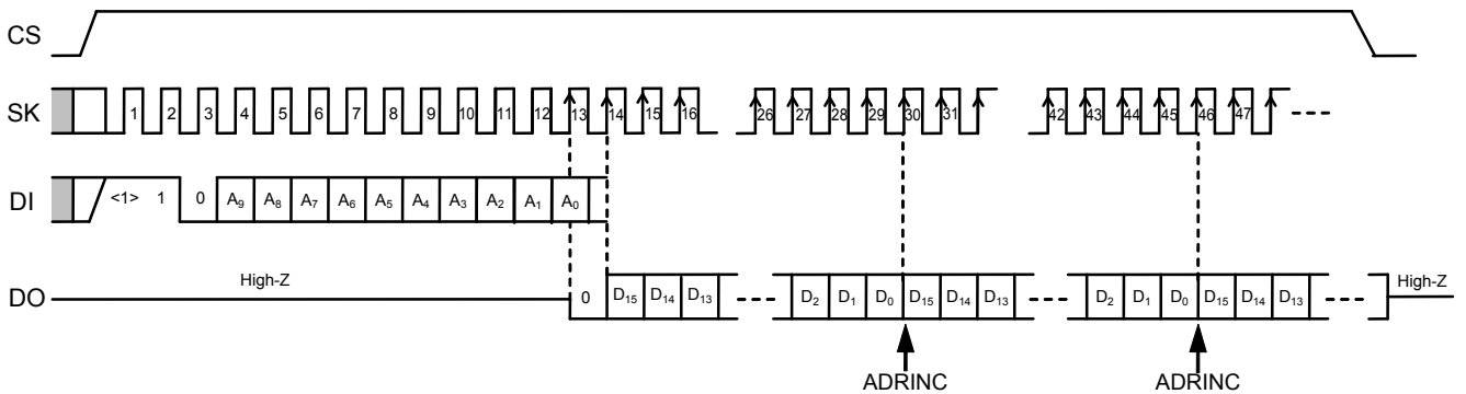
Figure 5 Read Timing
