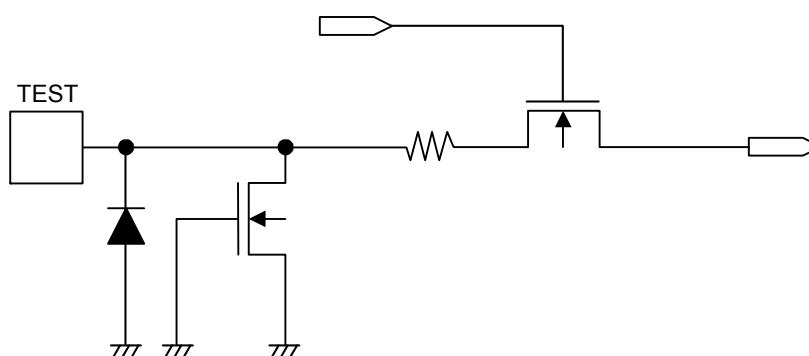
Figure 16 TEST Pin
