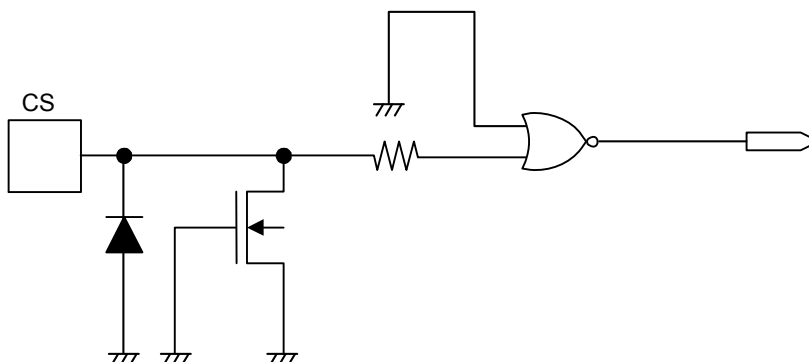
Figure 14 CS Pin
